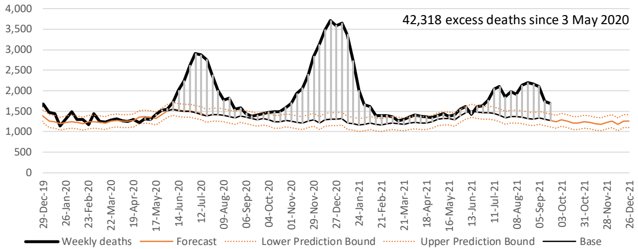
Eastern Cape weekly deaths from natural causes : 29 Dec 2019 - 25 Sep 2021
