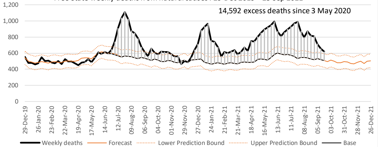
Gauteng weekly deaths from natural causes : 29 Dec 2019 - 25 Sep 2021
